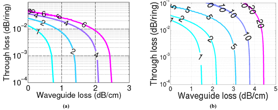
Fig. 3. Optical power requirement contours for: (a) core-to-DRAM LMGs network in Fig. 1, (b) core-to-core Clos network in Fig. 2,
