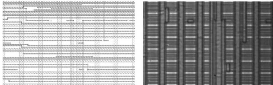
Fig. 9. Plot and corresponding photomicrograph showing chip power grid and routing. Metal layers 5 (horizontal) and 6 (vertical) are visible, and the height is seven standard-cell rows (about 35\ \mu\text{m} ).
